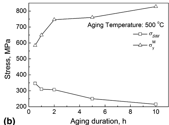
Fig. 4 Effects of aging temperature (a) and duration (b) on \sigma_y^M and \sigma_{SIM} . The data of the solution-treated sample are also given as dashed line
