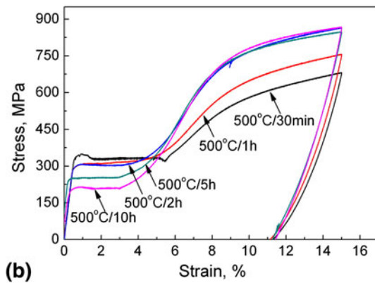
Fig. 3 Stress-strain curves of the TiNiV alloys solution-treated and aged at different temperatures for 30 min (a) and at 500 °C for different durations (b). The testing temperature was room temperature
